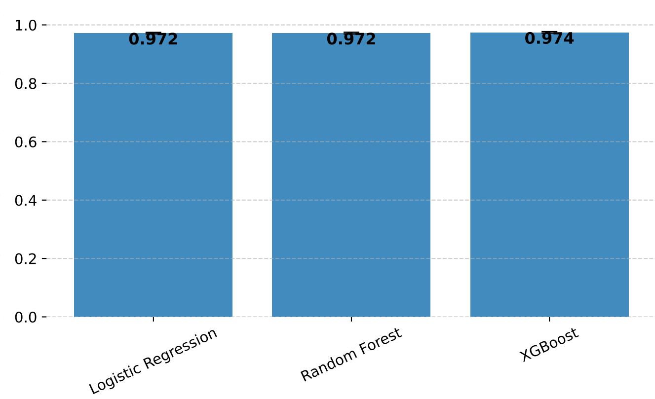
Recall
